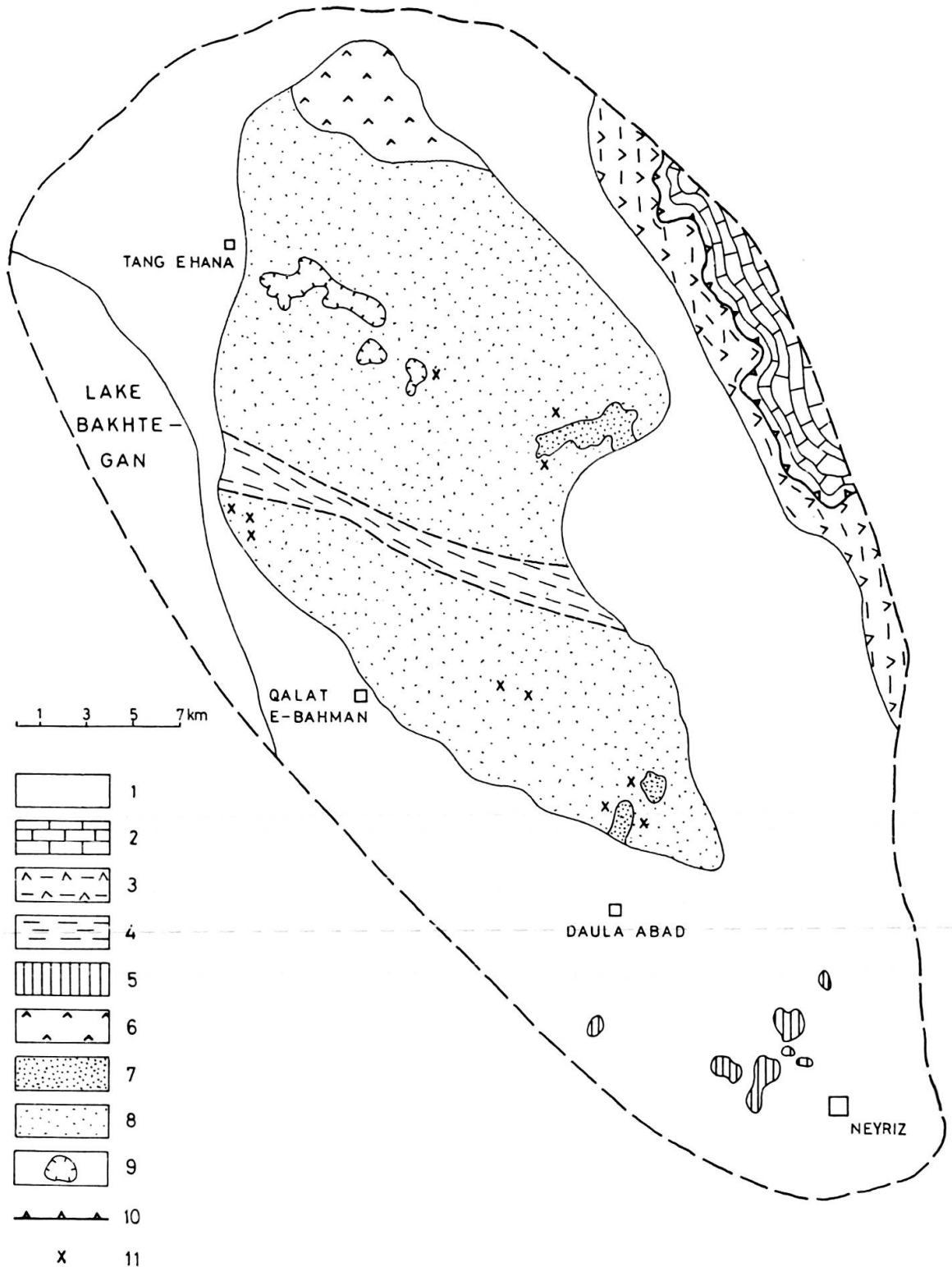
FIG. 2. — Geologic sketch map of the southeastest parts of the Neyriz ophiolitic complex. 1. Quaternary; 2. Cretaceous-Tertiary limestones; 3. Volcanic rocks with chert, limestone and shale; 4. Chert and limestone; 5. "Melange"; 6. Diabase; 7. Gabbro; 8. Harzburgite; 9. Marble nappes; 10. Main Zagros thrust; 11. Frequent rodingite occurrences.
