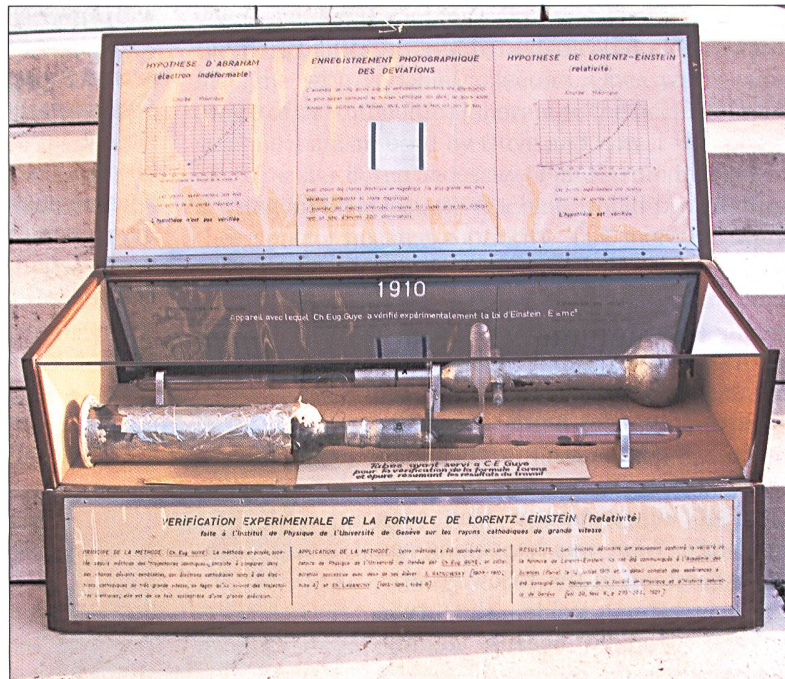
Fig. 7. The wooden cabinet with Guye's two cathode ray tubes (courtesy of The Geneva Science Museum).
