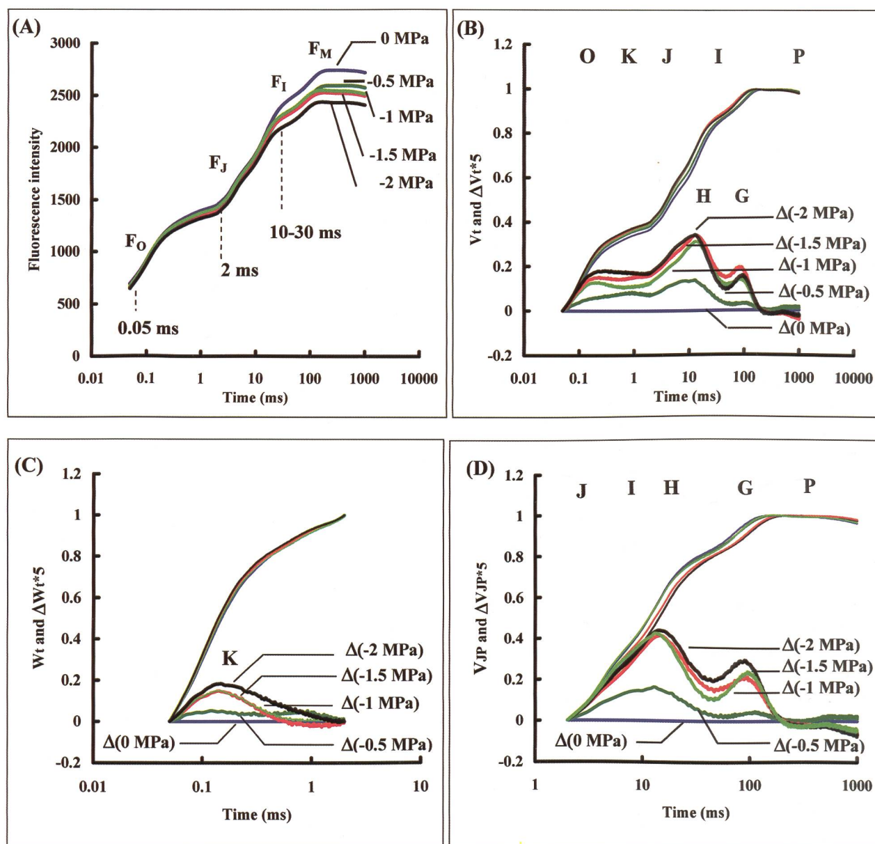
Fig. 2. An example of chlorophyll a polyphasic fluorescence rise O-J-I-P, exhibited by Ait Baha under different PEG-6000 solutions (0 MPa, -0.5 MPa, -1 MPa, -1.5 MPa and -2 MPa). The transients were plotted on a logarithmic time scale from 50 \mu s to 1 s (Fig. 2A). The marks refer to the selected fluorescence data used by the JIP-test for the calculation of structural and functional parameters. Fig. 2B shows the relative variable fluorescence ( V_t ) and ( \Delta V_t ) of the different fluorescence transients. Fig. 2C shows the relative variable fluorescence ( W_t ) and ( \Delta W_t ) in single turn-over phase (O-J). Fig. 2D shows the relative variable fluorescence ( V_t^{MT} ) and ( \Delta V_t^{MT} ) in multiple turn-over phase (J-P).
