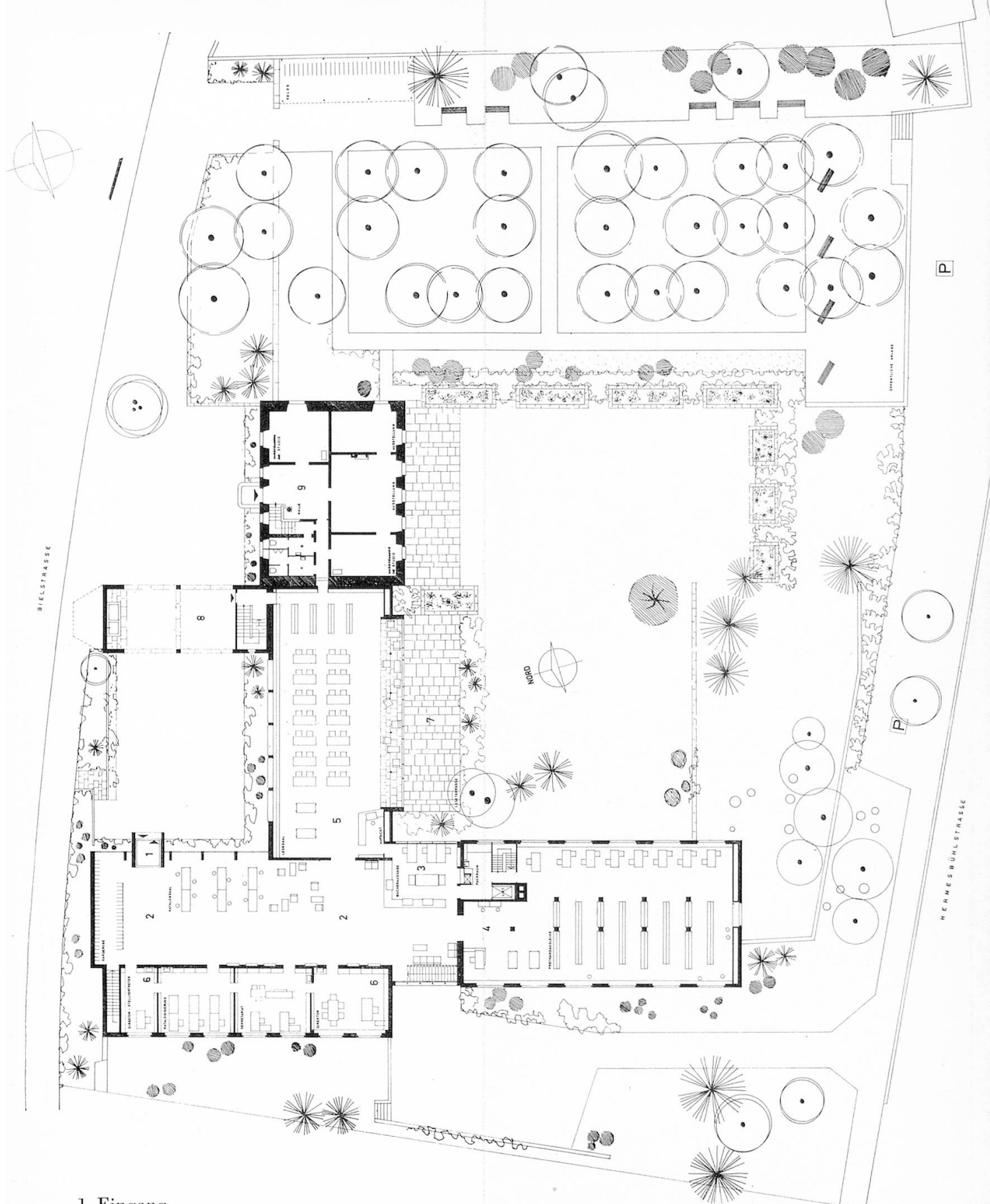
Grundriß Erdgeschoß
