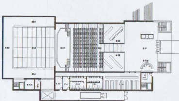
B PIANO TERRENO TEATRO 0.00/+1.20
