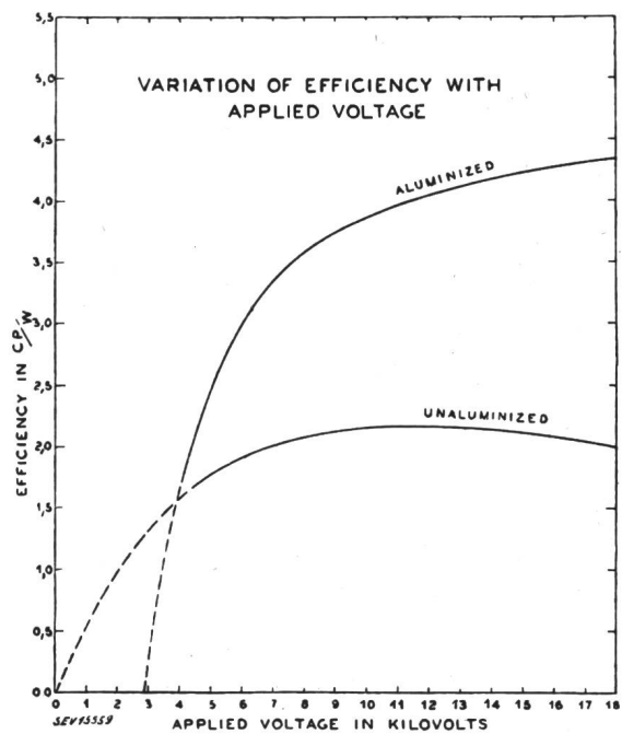
Fig. 19 Conversion Efficiency of 12-inch Kinescopes with and without Metal Film as Function of Operating Voltage
