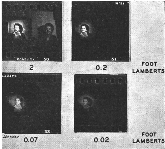
Fig. 17 Comparison of Sensitivity of Image Orthicon and Motion Picture Film
