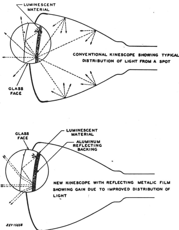
Fig. 18 Effect of Deposition of Reflecting Film on Kinescope Screen on Light Emission
