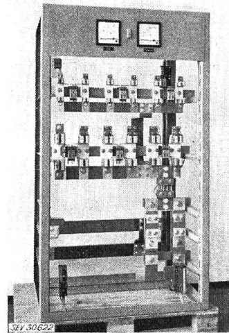
Fig. 10 Distribution 48 V
