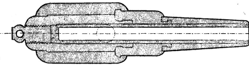
WROUGHT IRON MUZZLE LOADING GUN 10 INCH 18 TONS
