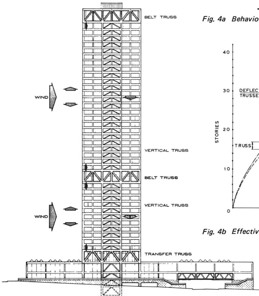
Fig. 3 East-West section showing lateral load resisting trusses
