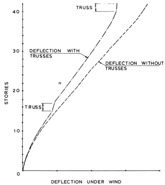
Fig. 4b Effectiveness of trusses in lateral resistance
