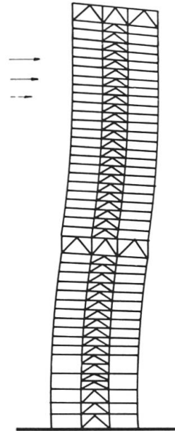
Fig. 4a Behaviour under lateral forces
