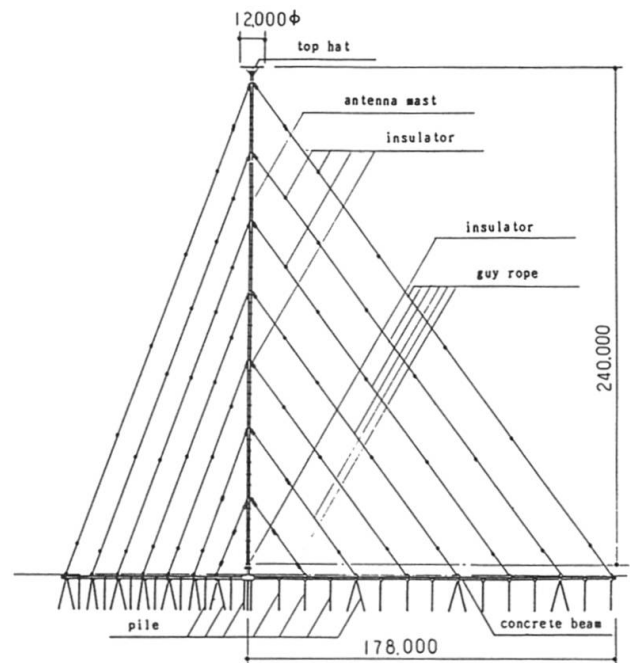
Antenna mast
