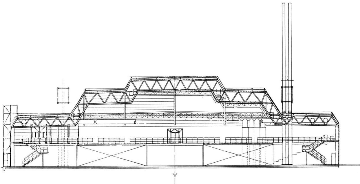
Fig. 2: Section
