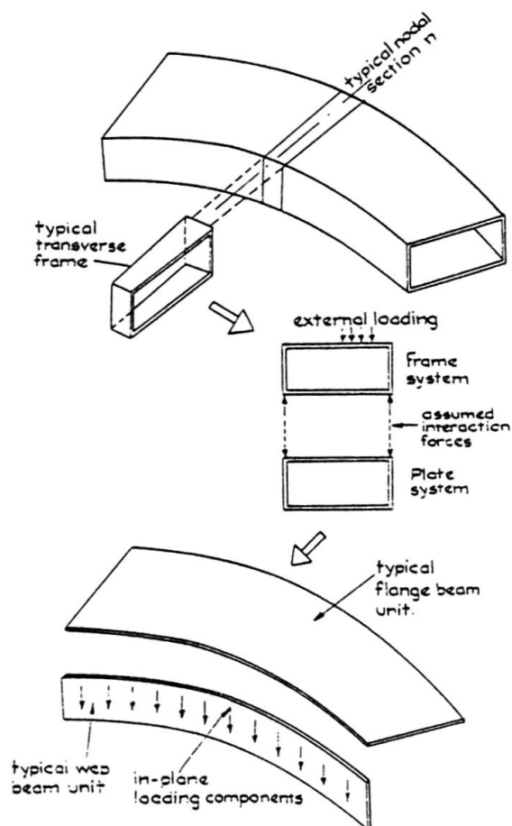
Fig. 2 Illustration of steps carried out in a typical nodal section analysis
