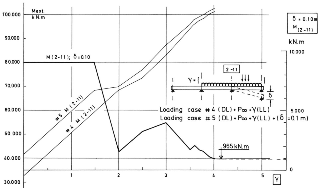
FIGURE 12 . - Evolution of the bending moment at the support cross-section (2.11), due to an abutment settlement, \delta .
