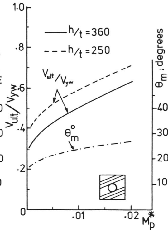
FIG. 2(b) PANEL OF ASPECT RATIO 1 HAVING A CUTOUT d/h=0.3
