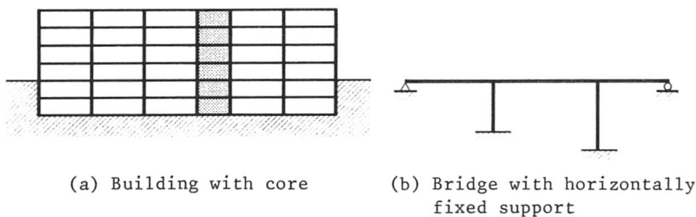
Fig. 2 Deformation Problems
