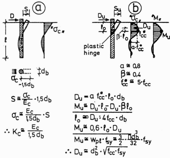
Fig. 9: Quasi-elastic (a) and plastic compressive (b) models for dowel action
