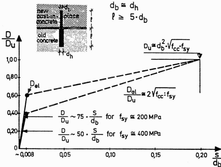
Fig. 10: Quasi-elastic and plastic compressive stage for dowels embedded in non-cracked concrete. The limit value s_u:d_b = 0,2 is based on data by J. Verdeyen and J. Gillet (1967) for piles in a cohesive soil
