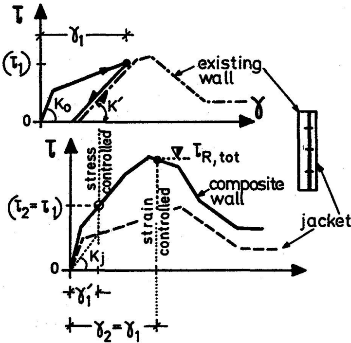
Fig. 46: Combination of existing R.C. wall (damaged at " \tau_1 "-shear level and unloaded) with a R.C. jacket; the composite wall is exposed to future stress \tau_2 = \tau_1 or to future strain \gamma_2 = \gamma_1
