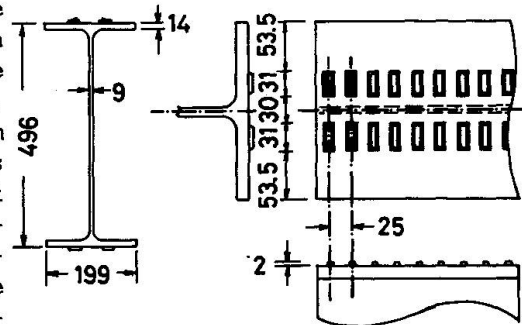
Fig.8 Embossed H-shape
