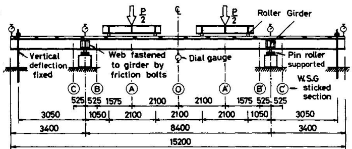
Fig.13 Ordinary span test in continuous beam
