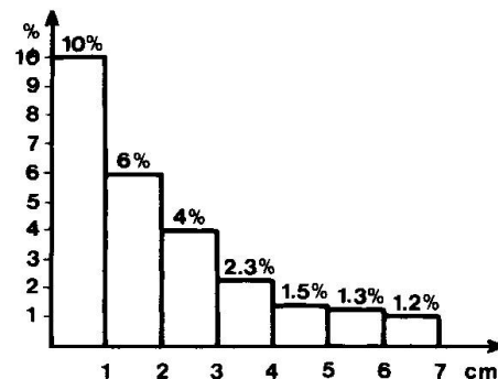
Fig 4. Diagram showing ion content compared with the quantity of cement from surface towards the interior of the Pag Bridge grider
