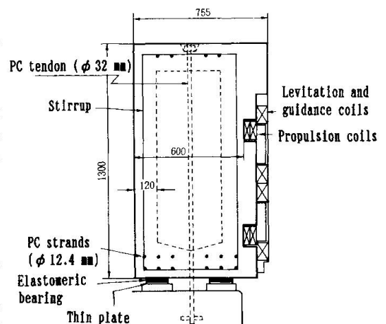
Fig.2 Cross section
