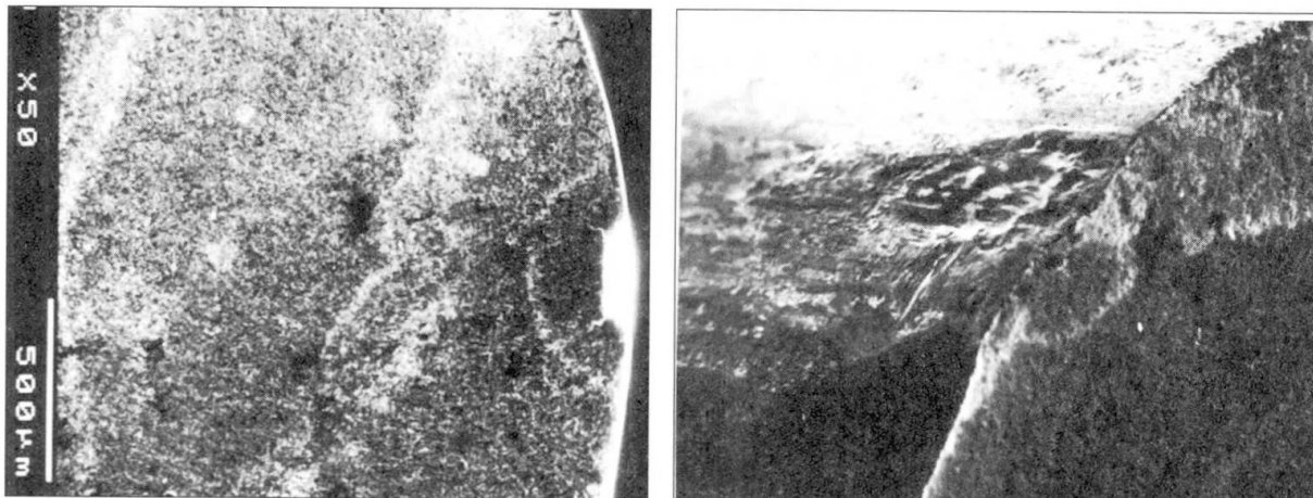
(A) Fatigue Fracture Surface (50 Magnifications)
