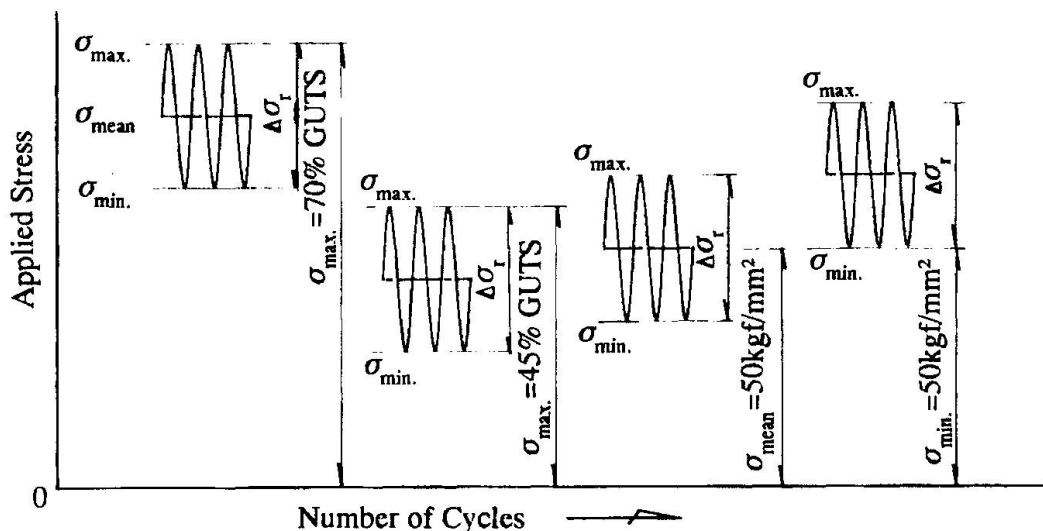
Fig. 2 Examples of the Definitions of Stresses in Fatigue Tests
