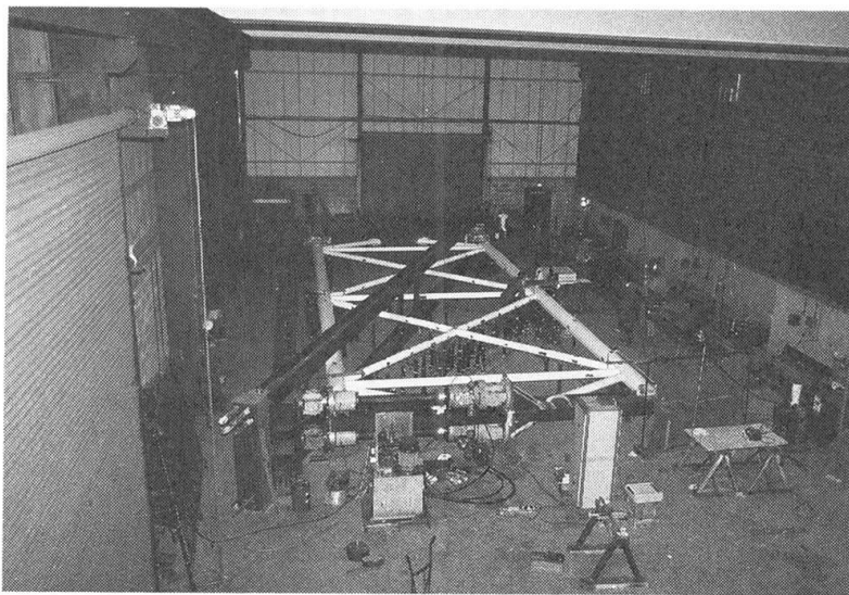
Fig. 3 View of Phase I frame test
