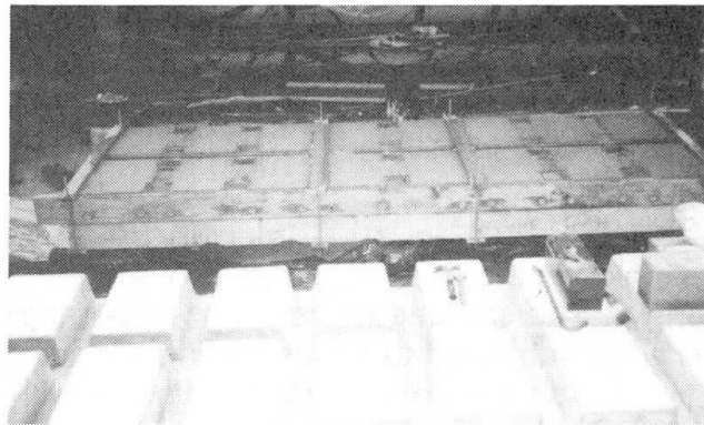
Fig. 8 In-situ shear tests of Hilti Jumbo Nails
