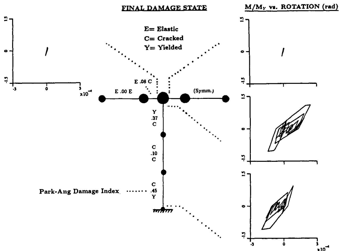
Fig. 5 Hysteresis damage for scaled PGA_H = 1g event
