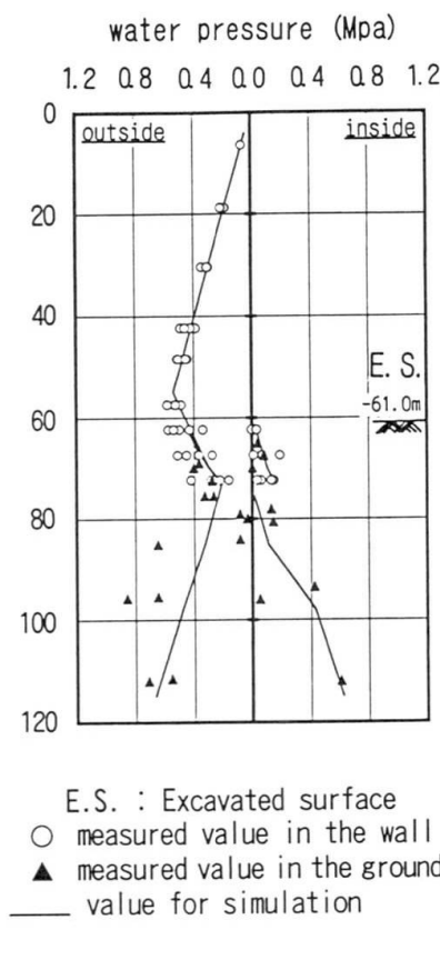
Fig4:Groundwater pressure distribution
