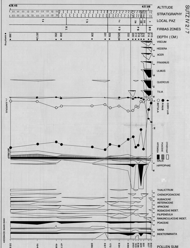
Figure 9. - Site IV, core 2/7, simplified pollen diagram for the Late Glacial and Early Holocene. See Fig. 3 for the location of the core and Fig. 8 for the legend.
