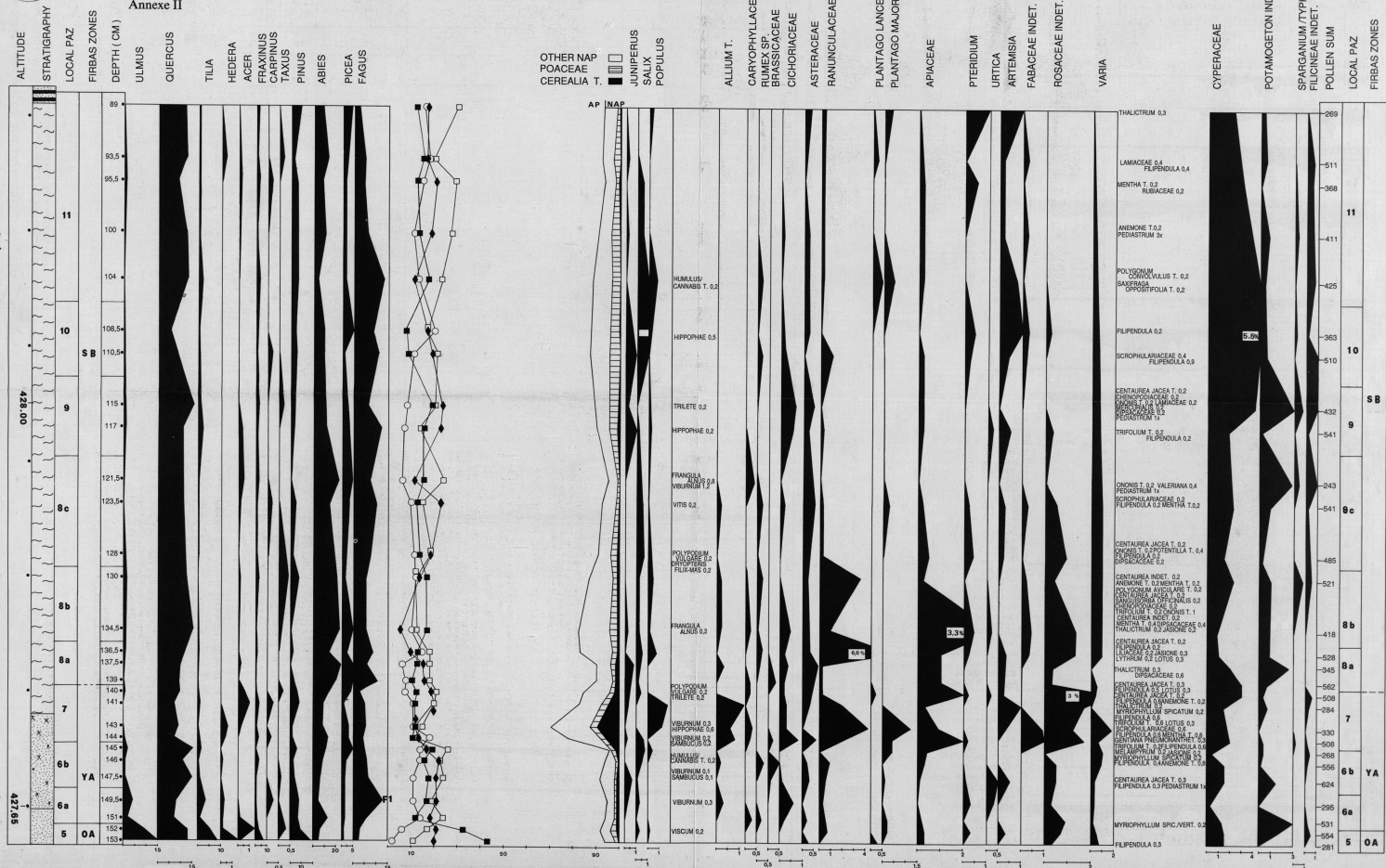
Figure 11. – Sutz IV, core 2/7, simplified pollen diagram of the Middle and Late Holocene. See Fig. 3 for the location of the core and Fig. 8 for the legend.
