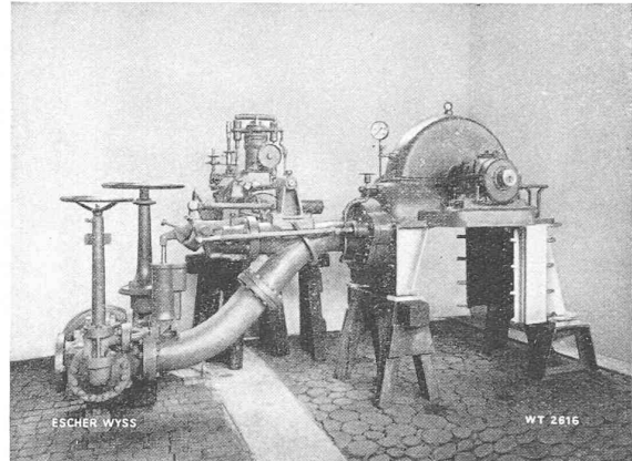
Fig. 5. — Turbine Pelton. H = 400 m P = 1150 ch n = 900 t : mn
