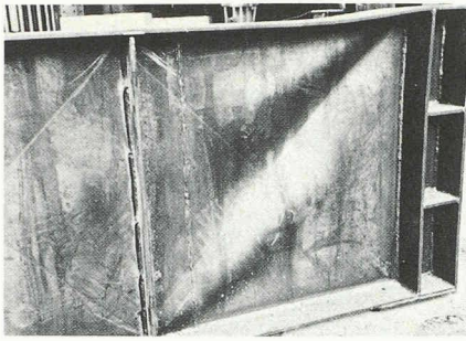
Fig. 3. — Typical collapse of a girder without longitudinal stiffener.
