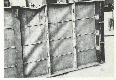
Fig. 5. — Typical collapse of a girder with three longitudinal stiffeners.
