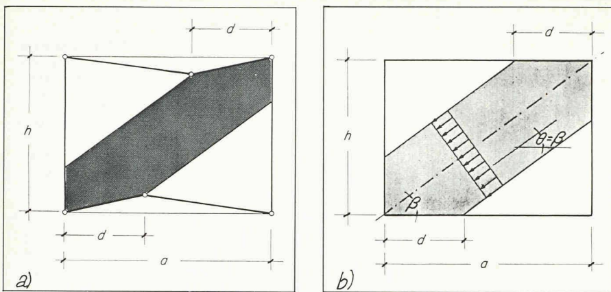
Fig. 1. — Collapse mechanism.
