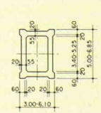
PILES 11-13
