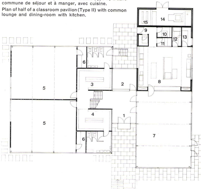
Erdgeschoß / Rez-de-chaussée / Ground floor 1:300
