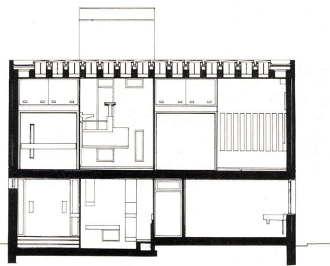
Querschnitt 1:200. Section transversale. Cross section.
