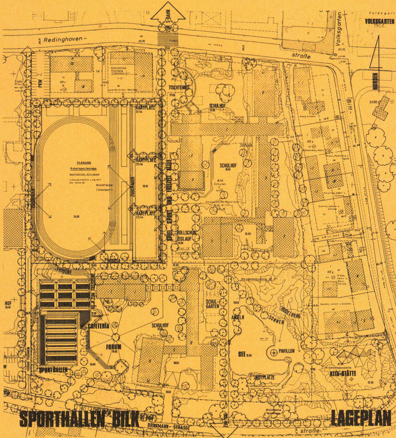
SPORTHALLEN BILK
