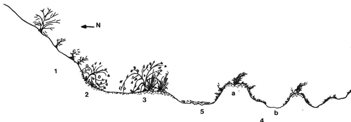
Fig. 2. – Wetland profile and wetland occupied by eolic sands:
