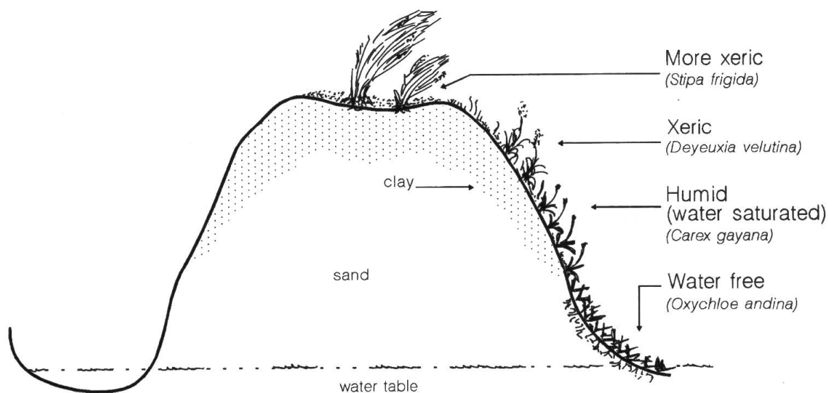
Fig. 3. – Cryogenic dome profile, with different xericity levels.
