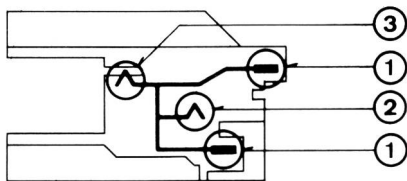
Fig. 7 Construction and schematic diagram of the connecting element ① Insulation displacing contact ② Isolating contact ③ Printed circuit board contact
