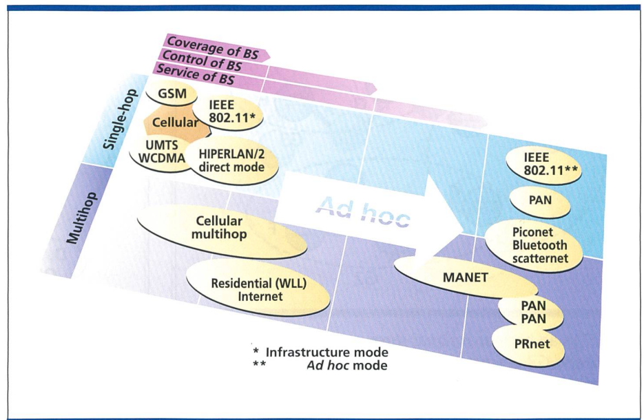
Fig. 2. Various wireless networks mapped to two independent aspects of ad hoc networking: the level of centralized control (horizontal), and the use of radio multihopping (vertical).
