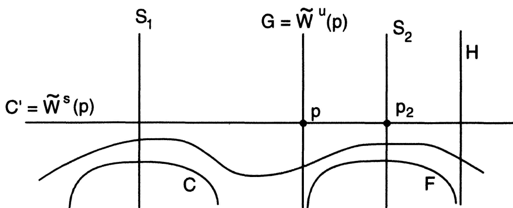
Figure 5. Producing a (3, 1) ideal quadrilateral.
