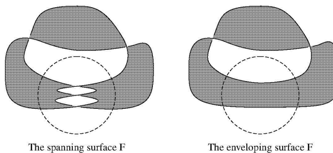
Figure 10. Visualizing the enveloping surface.
