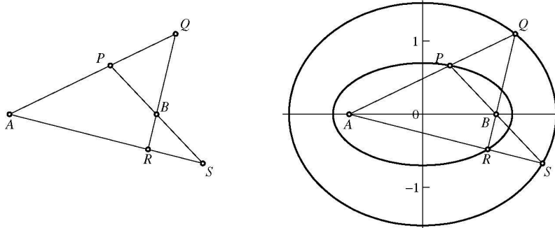
Fig. 3.1 Urquhart's theorem
