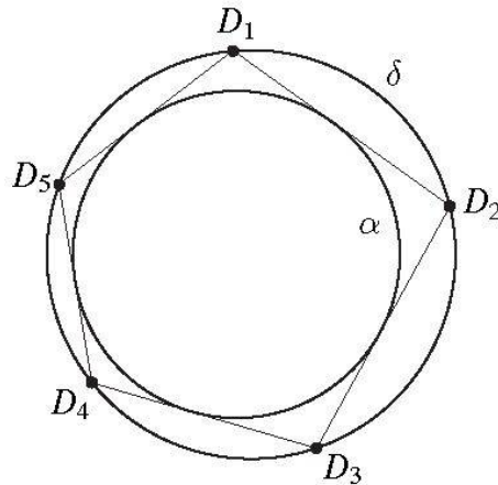
Fig. 1 Poncelet theorem
