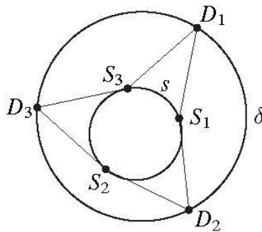
Fig. 3 Zigzag theorem
