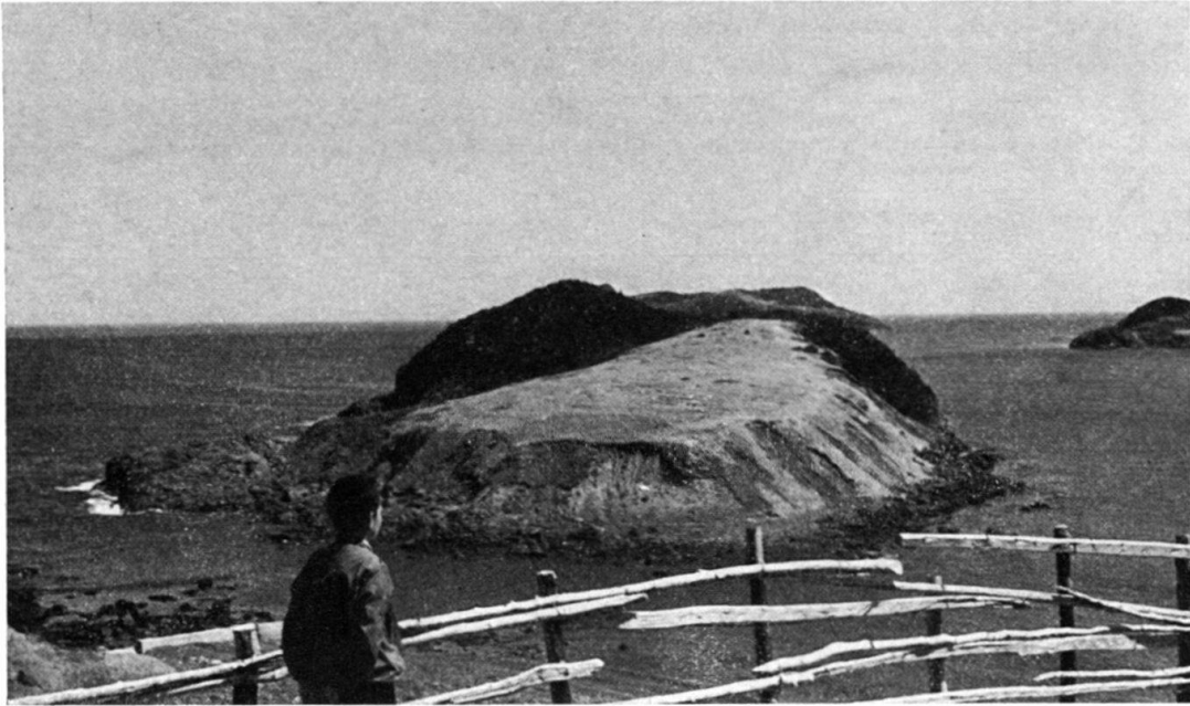
Fig. 15. Wave erosion of glacial drift in moderately sheltered position. The 'beach' is composed essentially of boulders washed out of the drift. The drift surface is smoothed because of solifluction. Island off Tor's Cove, about 25 miles (40 kilometres) south of St. John's, Avalon Peninsula.
