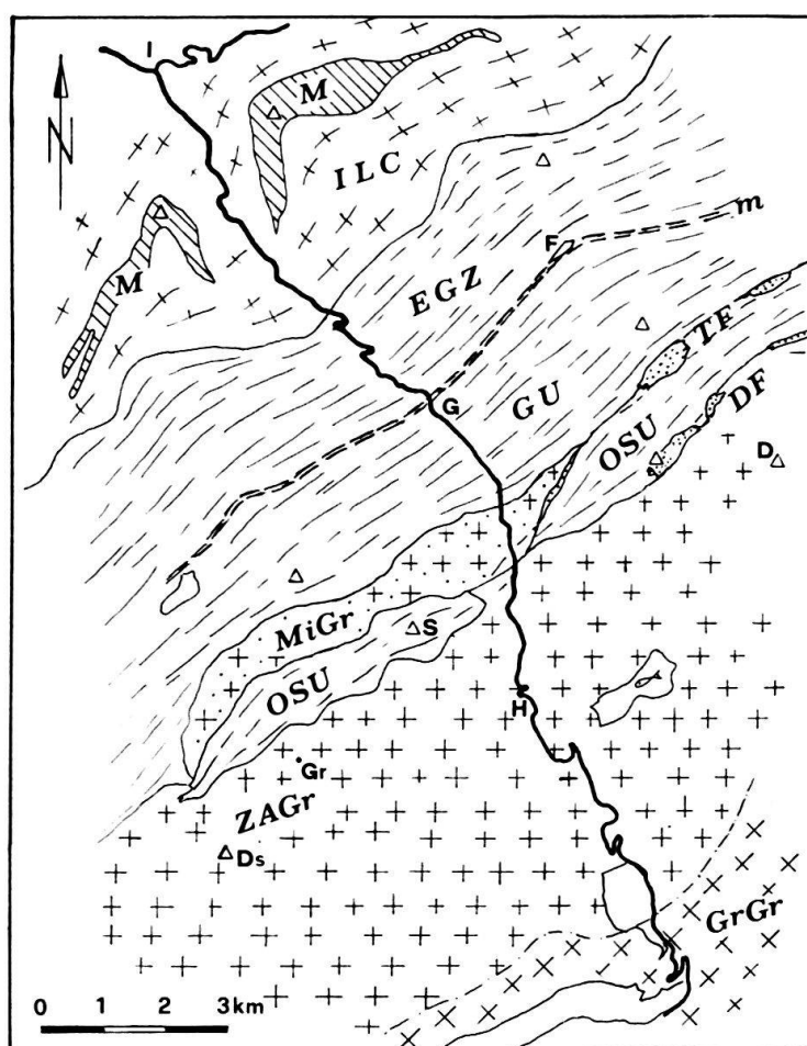
Fig. 3. Tectonic sketch map of the Oberhasli area. Localities: I = Innertkirchen, G = Guttannen, H = Handegg, F = Furtwangsattel, D = Diechterstock, Gr = Gruebenhütte AACB, Ds = Diamantstock. Geologic units: ILC = Innertkirchen–Lauterbrunnen Crystalline Complex, M = Mesozoic rocks, EGZ = Erstfeld Gneiss Zone, GU = Guttannen Unit, OSU = Ofenhorn–Stampfhorn Unit, TF = Triftgletscher-Fm, DF = Diechtergletscher-Fm, ZAGr = Central Aar Granite, MiGr = Mittagflue Granite, GrGr = Grimsel Granodiorite, m = mylonite zones.
