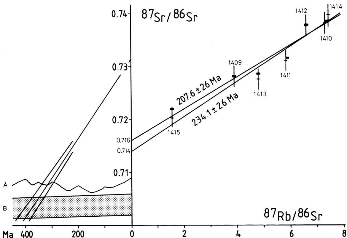
Fig. 8. Combined Sr-evolution and Compston-Jeffery diagram. The two isochrons were obtained during two measurement periods: 1974 data are indicated by large crosses, 1986 data by filled rectangles. The Sr-evolution line of the granitic rock crosses the seawater line (A) of BURKE et al. (1982) at about 315 Ma, the upper mantle limit (B; FAURE 1977) at about 350 Ma, the two points defining the lower and upper limit for the emplacement age.
