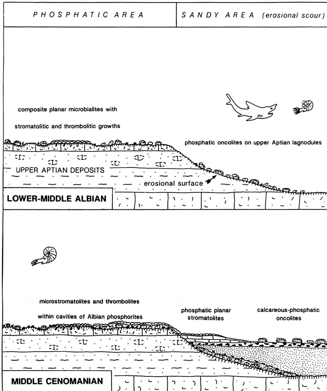
Fig. 20. Schematic reconstruction (without scale) of the mid-Cretaceous deposits and their microbialites in the Combe aux Puaires outcrop, Haut-Giffre massif (Haute-Savoie). Explanations in the text.
