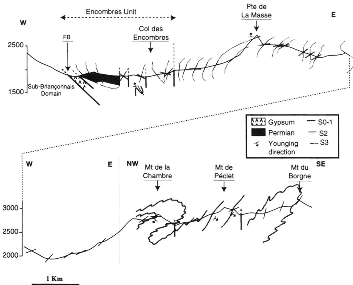
Fig. 4. Schematic cross-section of the ZHB stressing the attitude of the successive schistosités.
