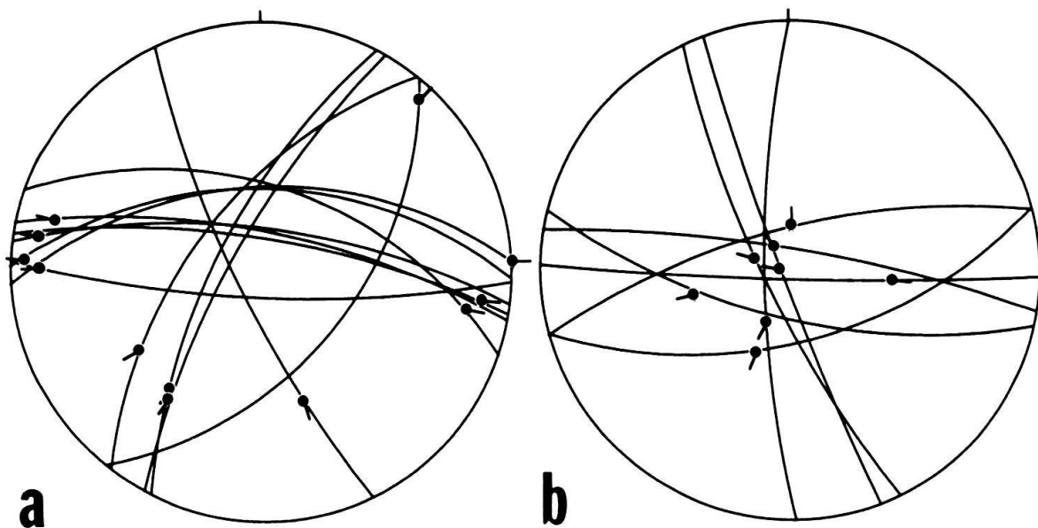
Fig. 7. Equal-area, lower-hemisphere stereographic representation of (a) strike-slip – mainly dextral – faults and (b) normal faults close to the PF zone near the Belleville valley.
