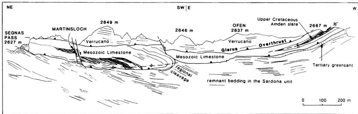
Fig. 5. Structure of the allochthonous Infrahelvetetic limestone beneath Tschingelhoren, which Pfiffner (1973) correlated with the parautochthonous Tschep-nappe; field of view 2 km.
