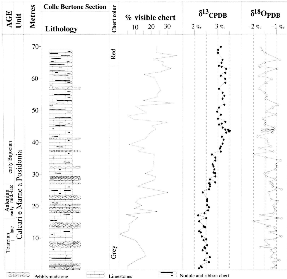
Fig. 3. Summary log of the Colle Bertone section. Lithology, visible chert percentage curve, \delta^{13}\text{C} and \delta^{18}\text{O} curves of bulk carbonates are simplified. For more details on lithology, sample locations, sample numbers and biostratigraphy see Plate 1.
