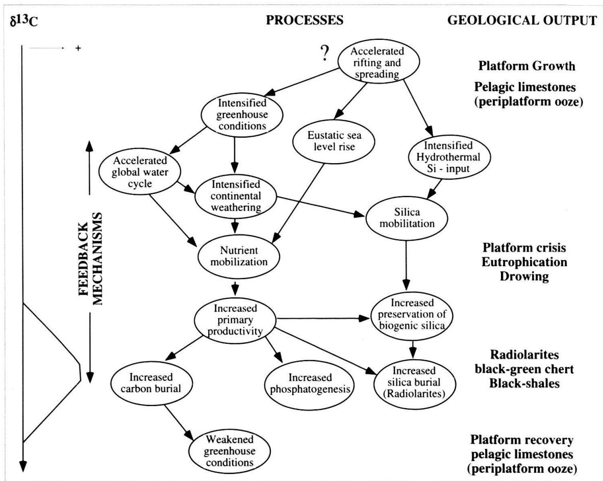
Fig. 13. Flow chart illustrating the links between carbon and silica cycles during the Middle-Late Jurassic, accelerated rifting and/or spreading supposedly was the endogenic force that triggered an exogenic regulation process through feedback mechanisms. It resulted in increased carbon and silica burial that re-established conditions like those prior to the endogenic perturbation. The time axis is from top to bottom without scale. Further explanations in the text (carbon cycle modified after Föllmi et al. 1994).
