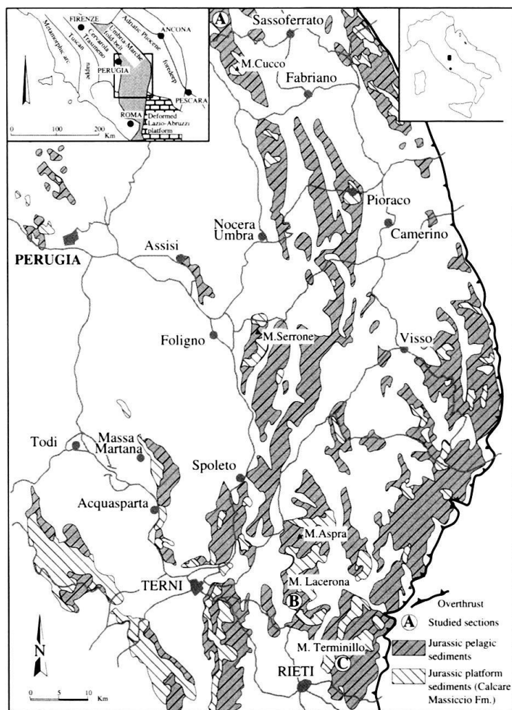
Fig. 1. Simplified geological map of the Umbria-Marche-Sabina Apennines with locations of sections A = Valdorbia; B = Colle Bertone; C = Terminillette.
