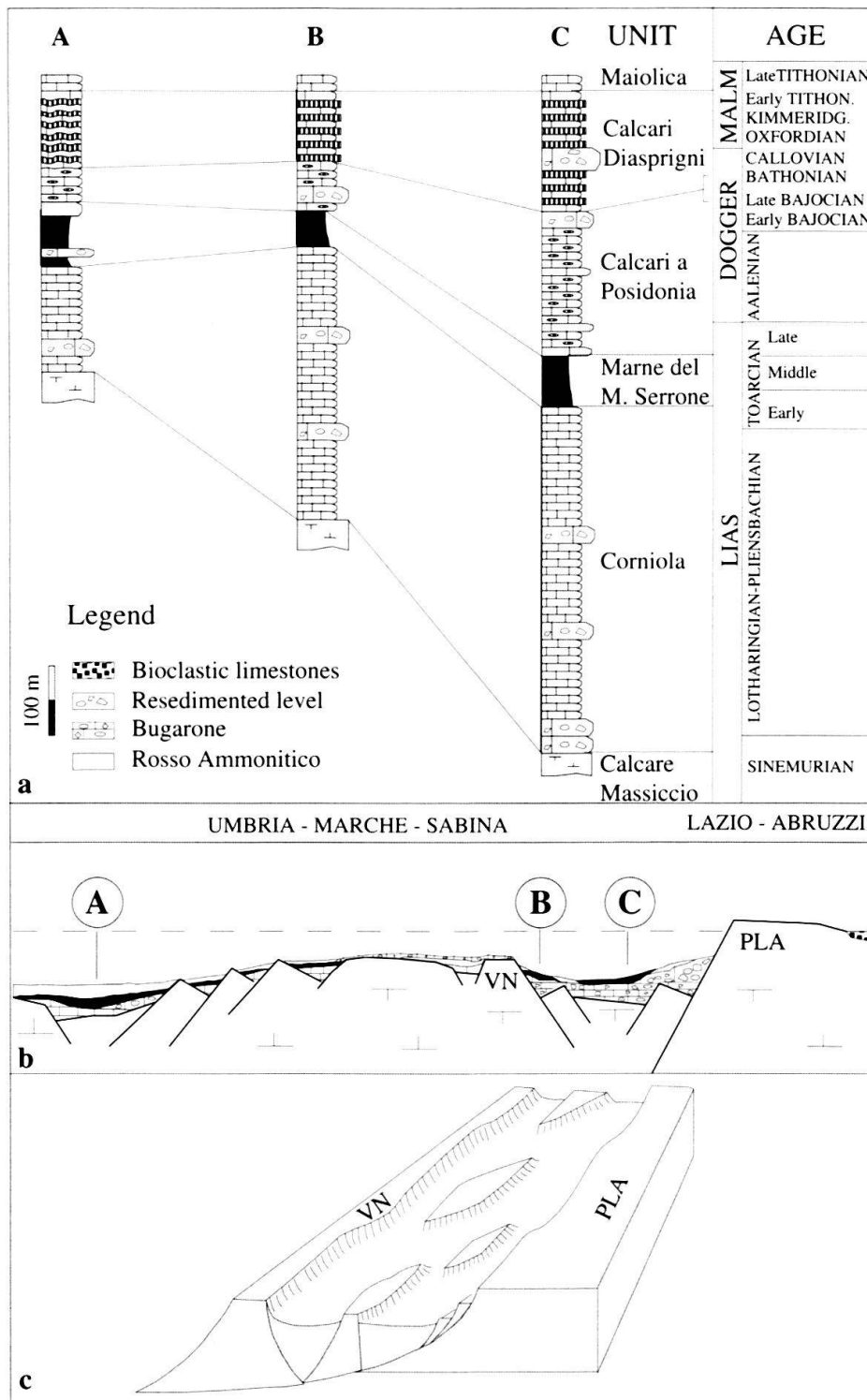
Fig. 2. (a) Simplified columnar sections and (b) paleogeographic transect of the Umbria-Marche-Sabina (UMS) Basin and the adjacent Lazio-Abruzzi (PLA) Platform. (A = Valdorbina, B = Colle Bertone, C = Terminilletto). The studied sections Colle Bertone and Terminilletto are located close to the area that represented the margin between the UMS Basin and the PLA Platform. This area was characterised by abundant carbonate resediment input from the platform, resulting in thicker and more calcareous sections than those out in the basin. (c) Schematic block model of the Lazio-Abruzzi Platform (PLA), and the proximal UMS Basin, The Valnerina Line (VN) formed a structural high during the Jurassic rifting (after Lavecchia 1985).
