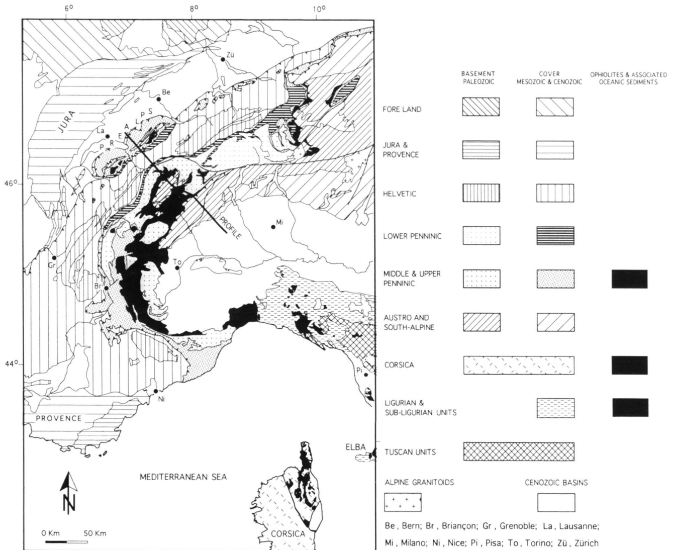
Fig. 1. Simplified tectonic map of the western Alps, Corsica and northern Apennines (modified from Escher et al. 1988 and Bigi et al. 1990).
