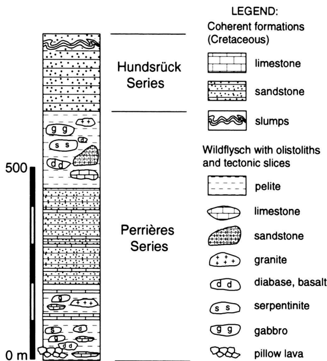
Fig. 3. Simplified stratigraphic section of the Gets nappe (modified from Caron & Weidmann 1967, Caron 1972 and Flück 1973).
