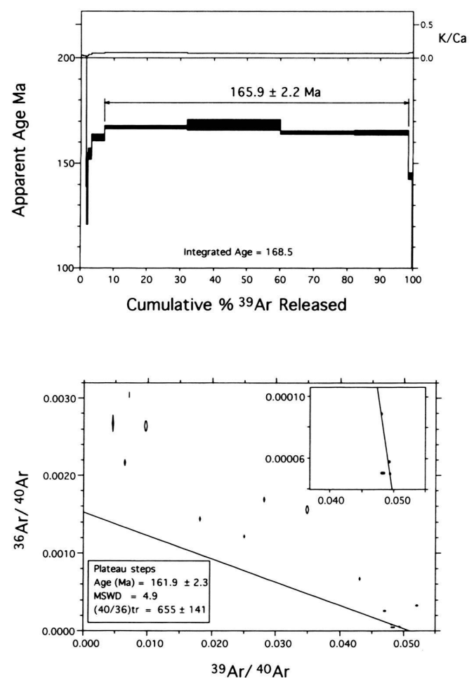
Fig. 5. ^{40}\text{Ar}/^{39}\text{Ar} age spectrum and isochron of the amphibole from gabbro MR3. Error ellipses on isochron are 1 sigma.
