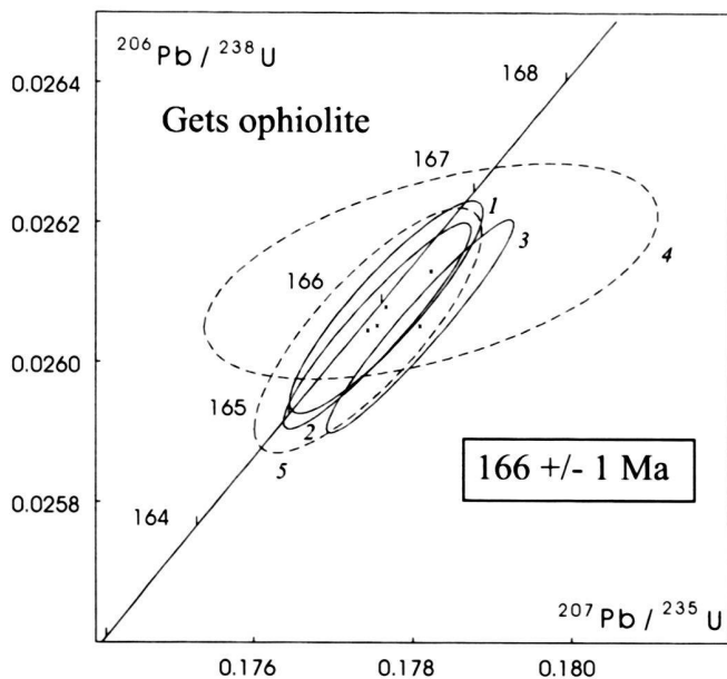
Fig. 4. U-Pb concordia diagram for zircons from gabbros MR3 and RB3. Ellipses are two sigma errors. Numbers refer to the zircon fractions listed in Tab. 1. Ellipses 1, 2, 3 relate to sample MR3, dashed ellipses (4,5) to sample RB3.
