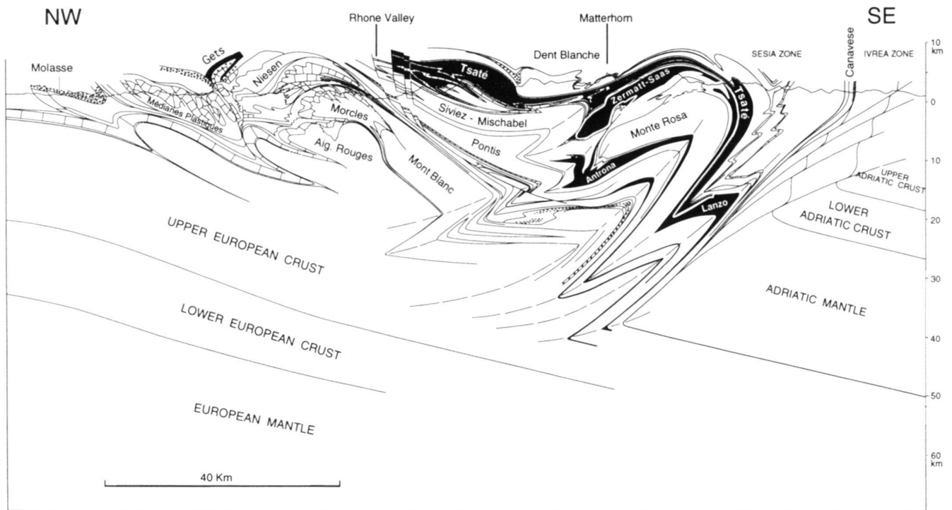
Fig. 2. Tectonic cross-section through the western Swiss Alps. Black: ophiolitic nappes (modified from Escher et al. 1993 and in press).
