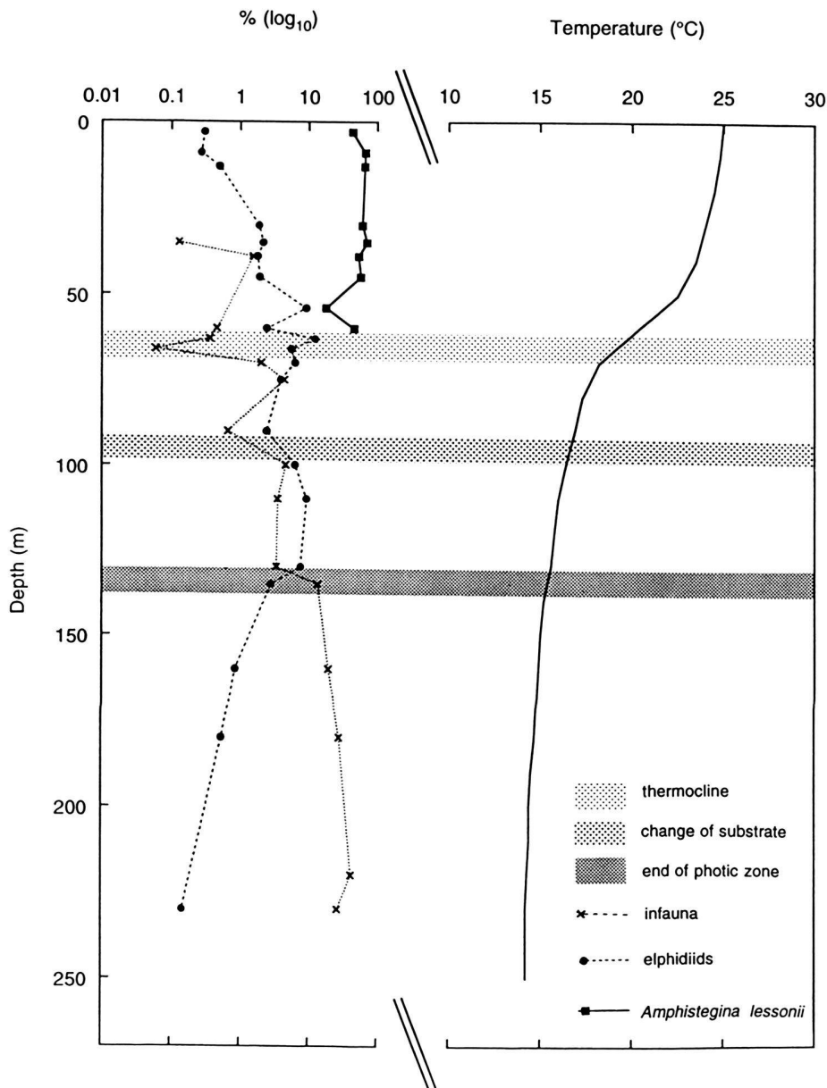
Fig. 2. Depth distribution of foraminiferal shells in the sediment from infaunal species, elphidiids and Amphistegina lessonii compared to depth gradient discontinuities in Eastern Crete. Frequencies are given in percent of total specimens in unitary sediment volumes. Note logarithmic scale of the frequency distribution.
