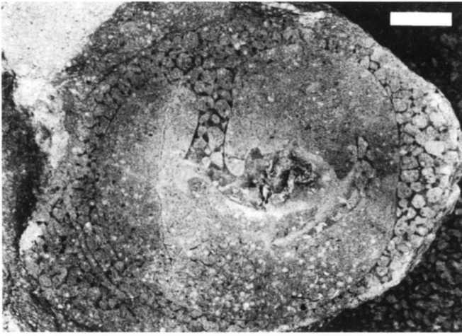
Fig. 1. Polished, oblique transverse section (viewed under water) of Campanile sp. A of Jung (1987) infested by Entobia sp. cf. E. laquea Bromley & D'Alessandro, 1984. This view shows the more apical end of the specimen. This is University of the West Indies Geology Museum specimen number UWIGM 1997.17. Scale bar represents 10 mm.
