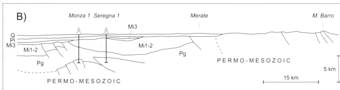
Fig. 1. A) Tectonic scheme of the western Southern Alps. Northern latitude and eastern longitude figures are reported in the frame; circles point at ENI/Agip wells (well names in italics ). B) Simplified seismic section along the N-S trace in A) (redrawn after Pieri & Groppi 1981); Pg = Paleogene; Mi1-2 = Lower to Middle Miocene; Mi3 = Upper Miocene (essentially Messinian); Pl = Pliocene; Q = Quaternary.
