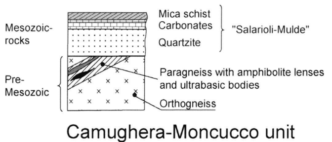
Fig. 3. Lithostratigraphic profile of the Antrona ophiolites taken at Alpe Ogaggia (see Fig. 2 for location and synthetic lithostratigraphic profile of the Camughera-Moncucco unit).
