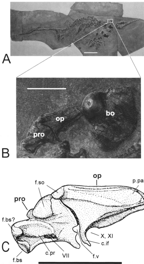
Fig. 1. Mixosaurus cf. cornalianus , PIMUZ T4848 (Middle Triassic, Grenzbitumenzone of Monte San Giorgio, Canton Ticino, Switzerland). A) Complete specimen in right lateral view, with framed left otic capsule and basioccipital bone. B) Left otic capsule in lateral view (left side of the photograph) and basioccipital bone in ventral view (right side of the photograph). C) Interpretative drawing of the left otic capsule as preserved, slightly compressed and seen in left lateral view. Abbreviations: bo, basioccipital; c.if, crista interfenestralis; c.pr, crista prootica lateralis; f.bs, f.bs?, facet and possible facet for basisphenoidal portion of parabasisphenoid; f.so, facet for supraoccipital; f.v, fenestra vestibuli or oval window; op, opisthotic, p.par, processus paroccipitalis; pro, proötic; VII, foramen nervi facialis; X, XI, foramen metoticum. Scale bars: A (10 cm); B, C (1 cm).
