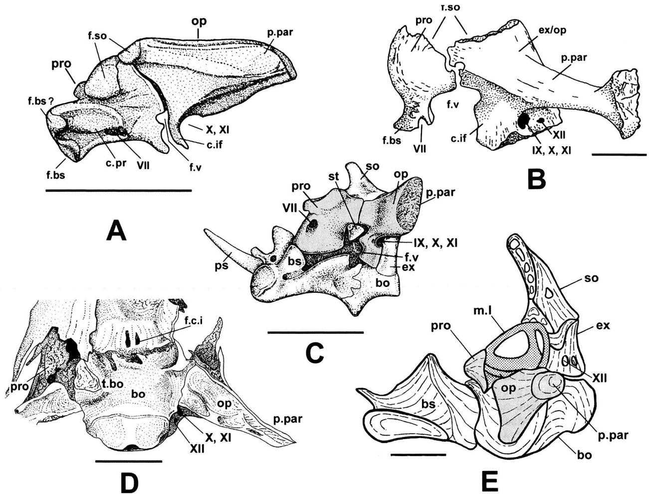
Fig. 2. Otic capsules and parts of braincases in ichthyosaurs and two other amniotes. A) Mixosaurus cf. cornalianus (PIMUZ T4848) left otic capsule in lateral view. B) The diapsid (sauroptrygian) Muraenosaurus leedsii (SEELEY 1874) from the Middle Jurassic of England, left otic capsule in lateral view (redrawn from Maisch 1998). C) The parareptile Procolophon trigoniceps OWEN 1876 from the Lower Triassic of South Africa, reconstruction of the braincase in left lateral view, with otic elements shaded in grey (redrawn from Carroll & Lindsey 1985). D) The basal ichthyosaur (cymbospondylid) Phantomosaurus neubigi (SANDER 1997) from the Middle Triassic of Germany, braincase in ventral view (redrawn from Maisch & Matzke in press). E) The derived ichthyosaur (ichthyosaurid) Ichthyosaurus communis CONYBEARE 1822 from the Lower Jurassic of England, reconstruction of part of the braincase in left lateral view with otic elements shaded in grey (redrawn from McGowan 1973). Abbreviations as in Fig. 1, and: bs, basisphenoid; ex, exoccipital; f.c.i, carotid foramen; m.l, membranous labyrinth; ps, parasphenoid; so, supraoccipital; st, stapes; t.bo, tuber basioccipitale; IX, X, XI, metotic foramen; XII, hypoglossal foramen. Scale bars: A-C (10 mm); D, E (20 mm).
